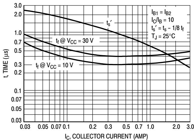
Figure 2. Turn-Off Time
